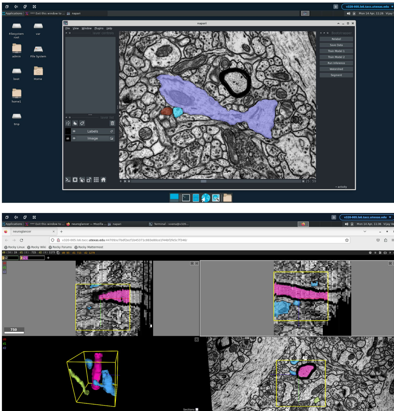
Fig. 3 The Napari application and Bootstrapper plugin. Top: Shown in use on 3dem.org. Sparse label annotations in color. Bottom: Screenshot of Neuroglancer viewer of same dataset illustrates ZY, ZX, and
